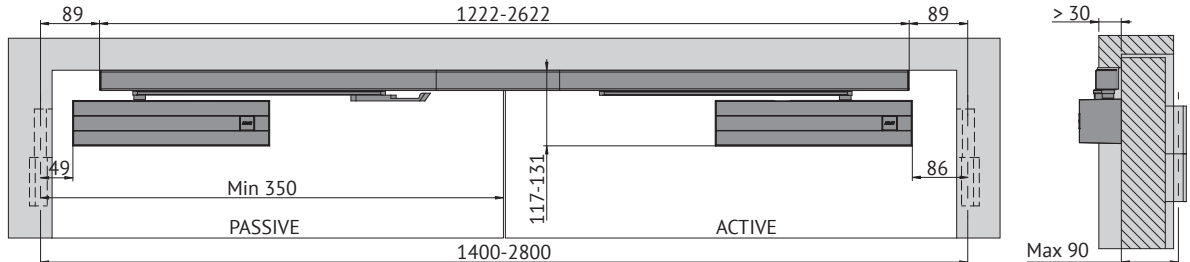
NON-HINGE SIDE WITH ANGLE MOUNTING PLATE
