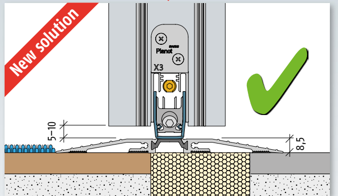
Renovation with thermal separated flat threshold F140 and Planet X3
