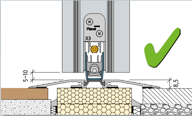
New building with thermal separated flat threshold F140 and Planet X3
