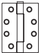
ANSI hole pattern (Template drilled)
